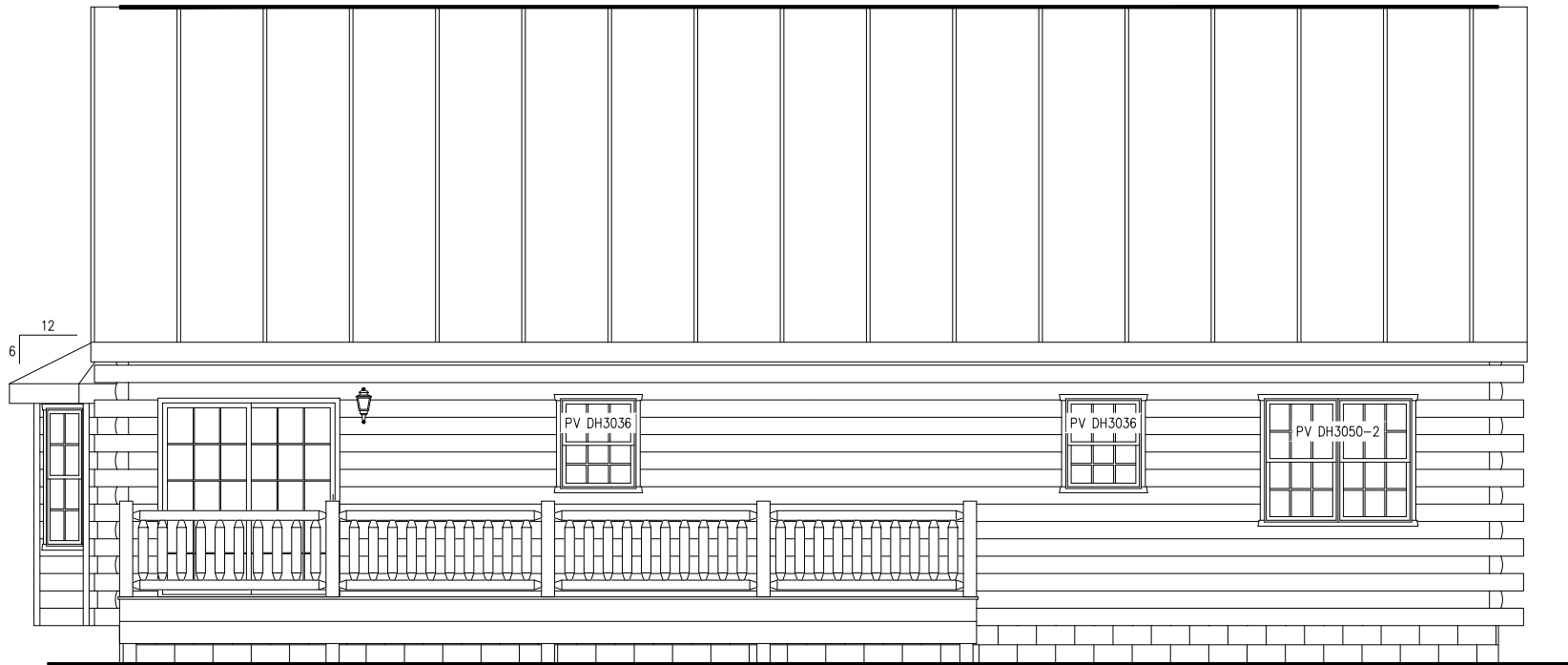
REAR ELEVATION
