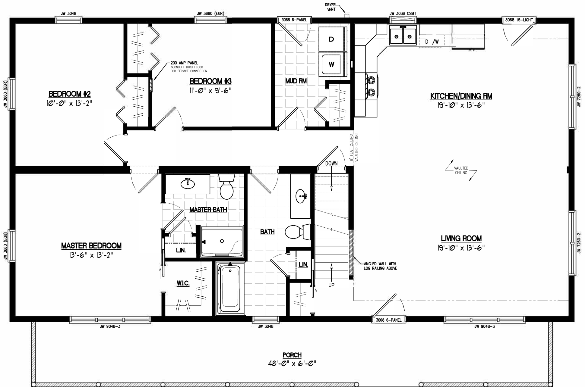
28x52 MOUNTAINEER DELUXE Plan #28MD1407
