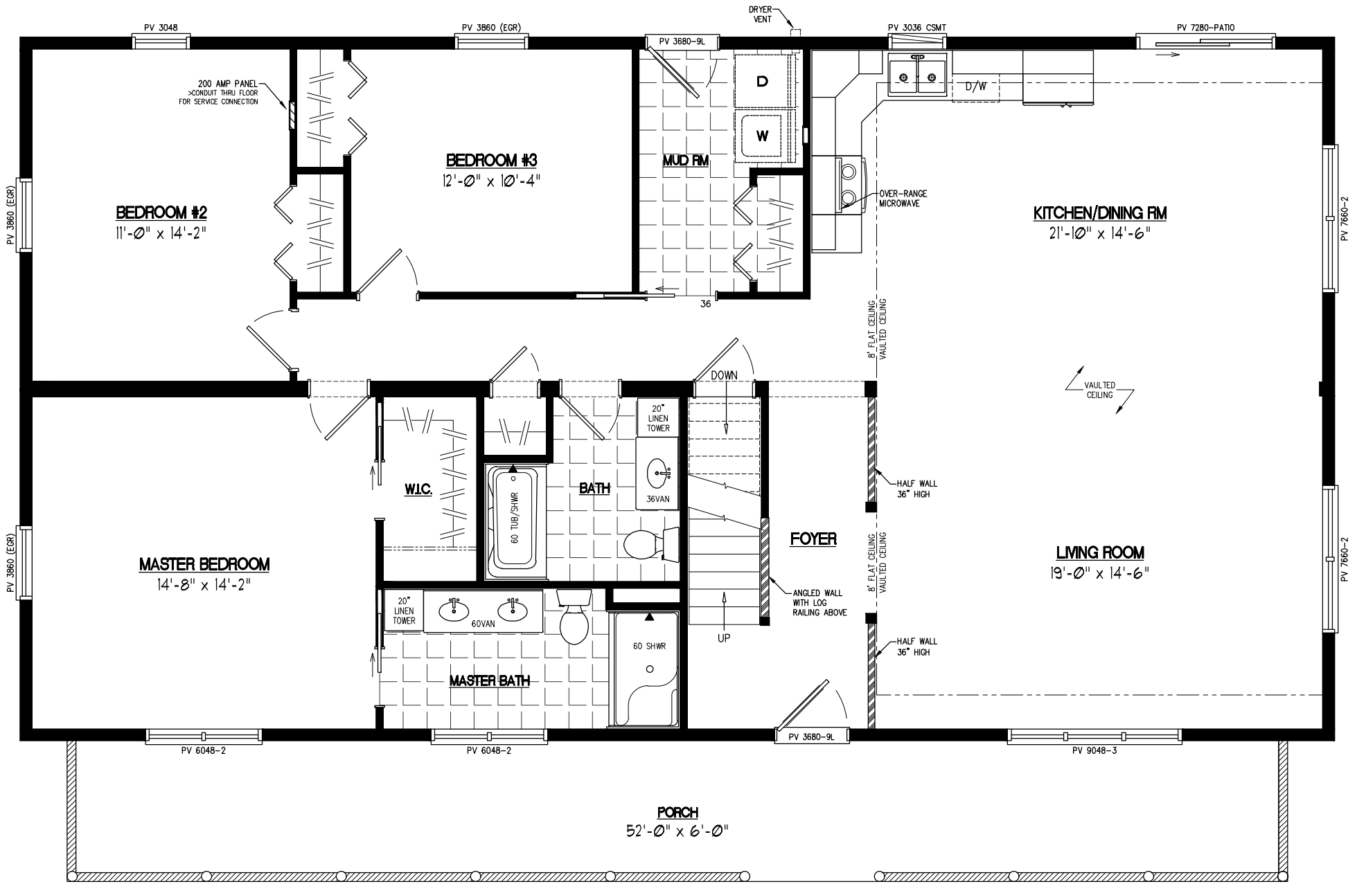
30x56 MOUNTAINEER DELUXE Plan #30MD1409
