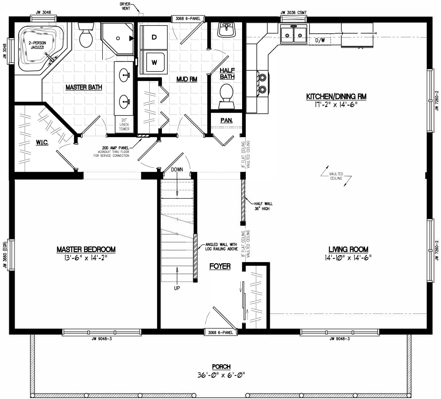
30x40 MOUNTAINEER DELUXE Plan #30MD1403
