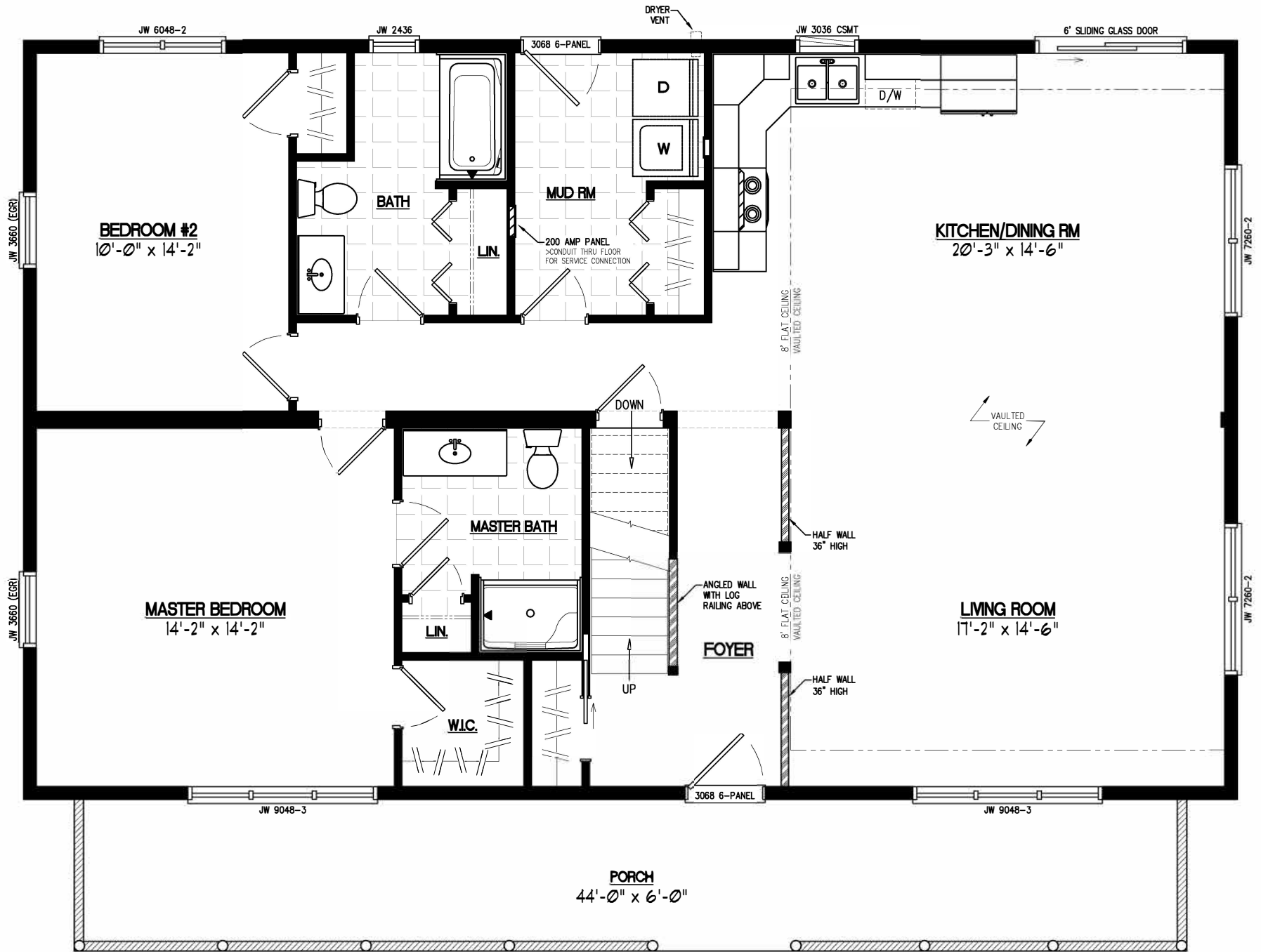
30x48 MOUNTAINEER DELUXE Plan #30MD1405
