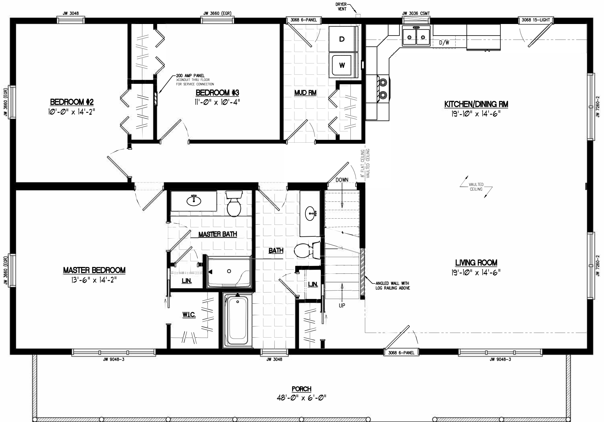
30x52 MOUNTAINEER DELUXE Plan #30MD1407
