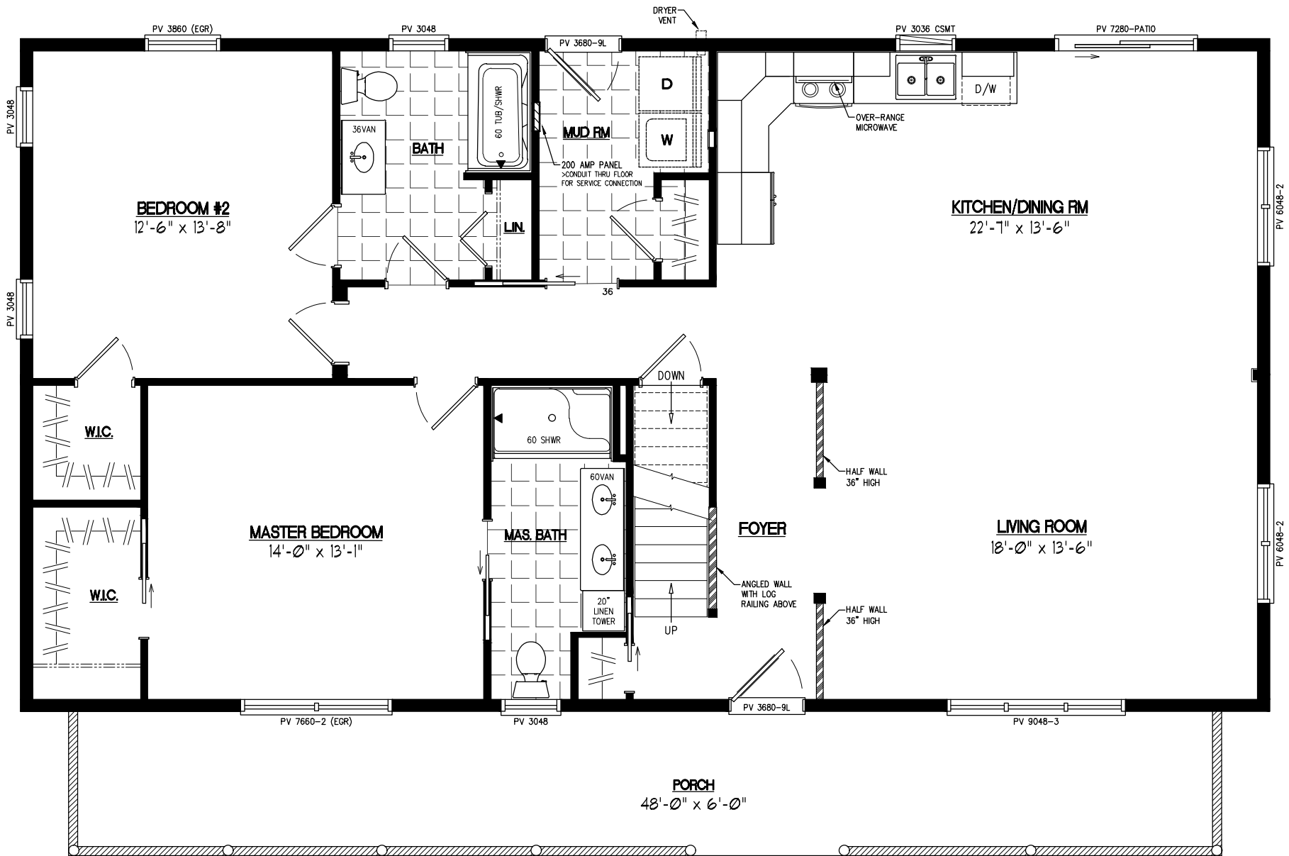
28x52 MOUNTAINEER Plan #28MR1306
