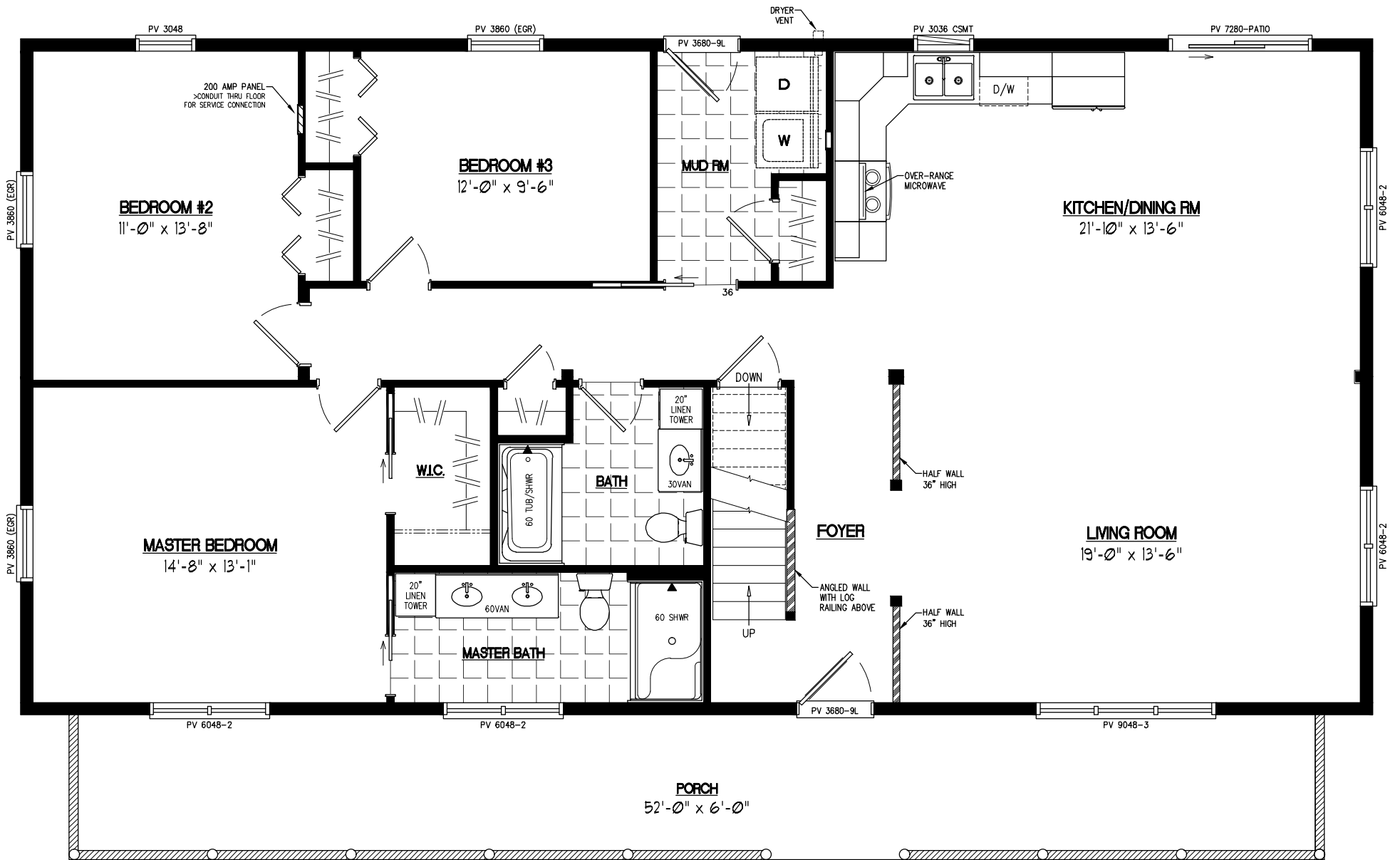
28x56 MOUNTAINEER Plan #28MR1309
