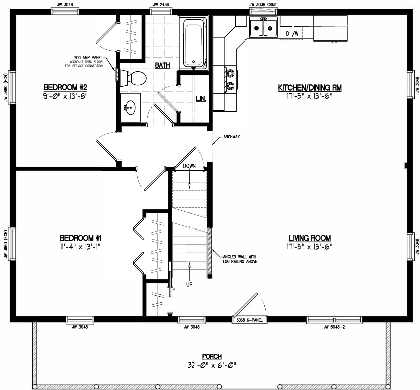
28x36 MOUNTAINEER Plan #28MR1302
