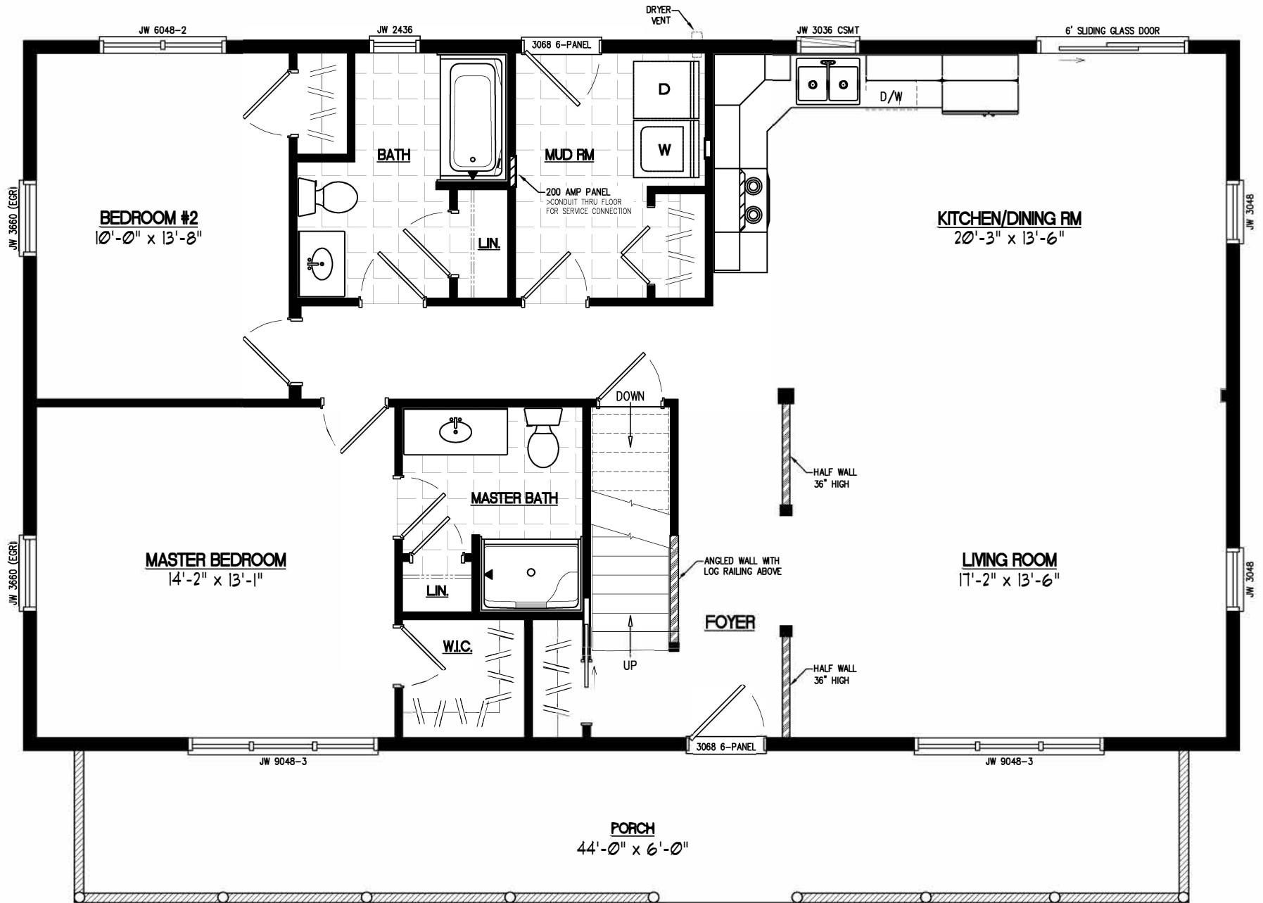
28x48 MOUNTAINEER Plan #28MR1305
