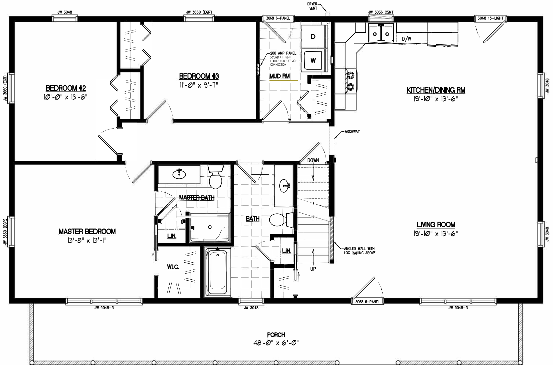
28x52 MOUNTAINEER Plan #28MR1307
