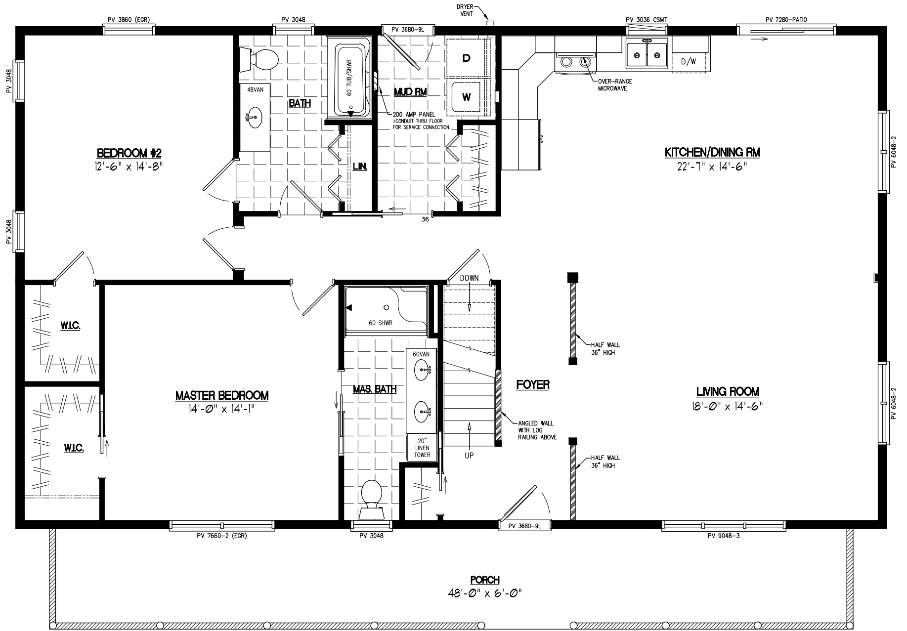
30x52 MOUNTAINEER Plan #30MR1306
