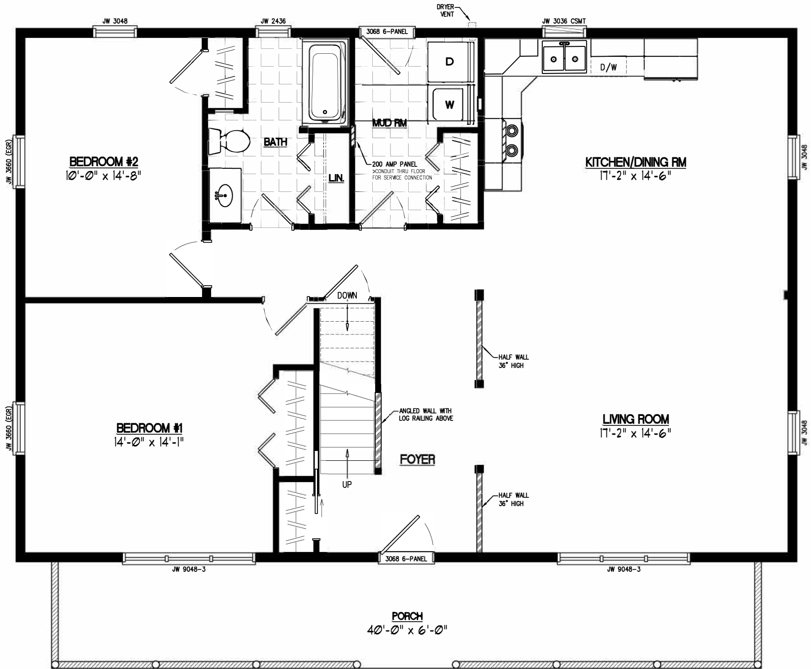
30x44 MOUNTAINEER Plan #30MR1304
