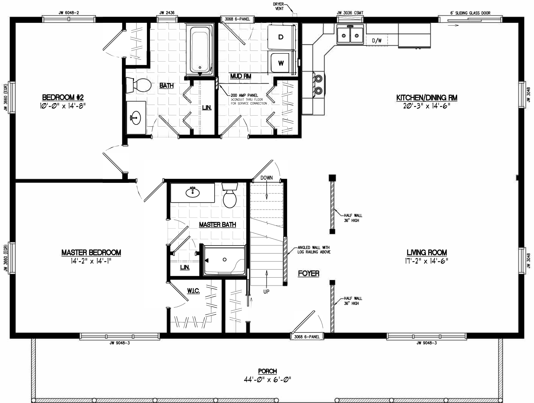
30x48 MOUNTAINEER Plan #30MR1305
