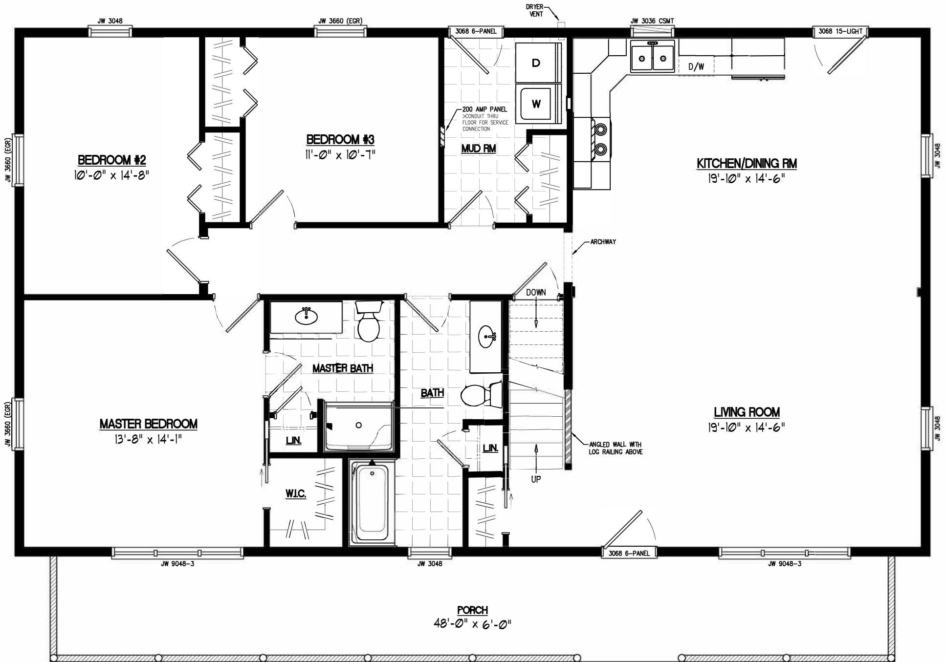
30x52 MOUNTAINEER Plan #30MR1307
