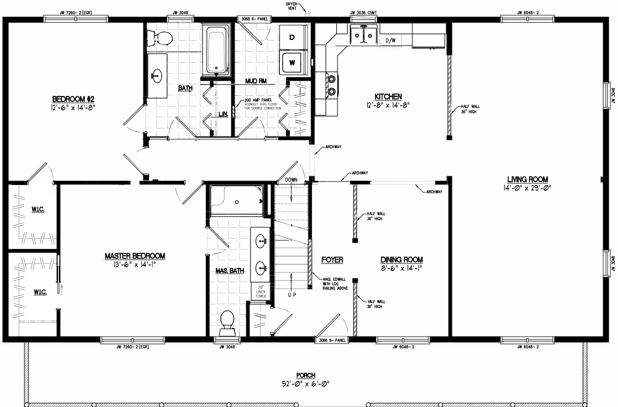
30x56 MOUNTAINEER Plan #30MR1308
