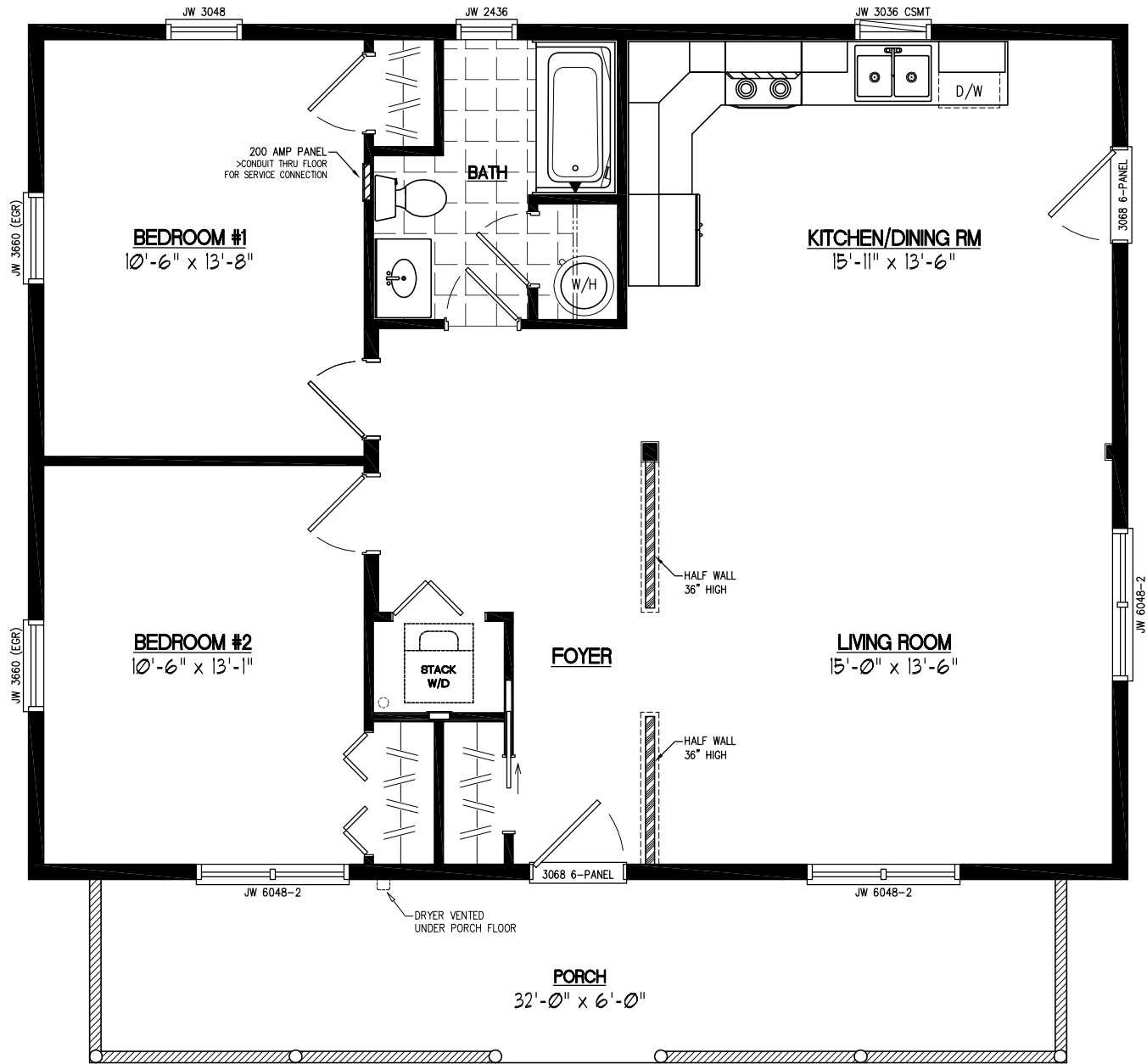
28x36 MUSKETEER Plan #28MK1502
