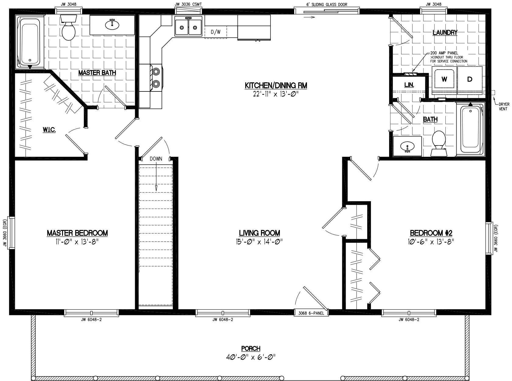
28x44 MUSKETEER Plan #28MK1504
