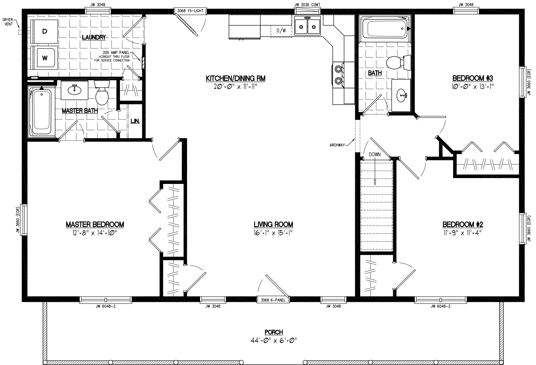
28x48 MUSKETEER Plan #28MK1505
