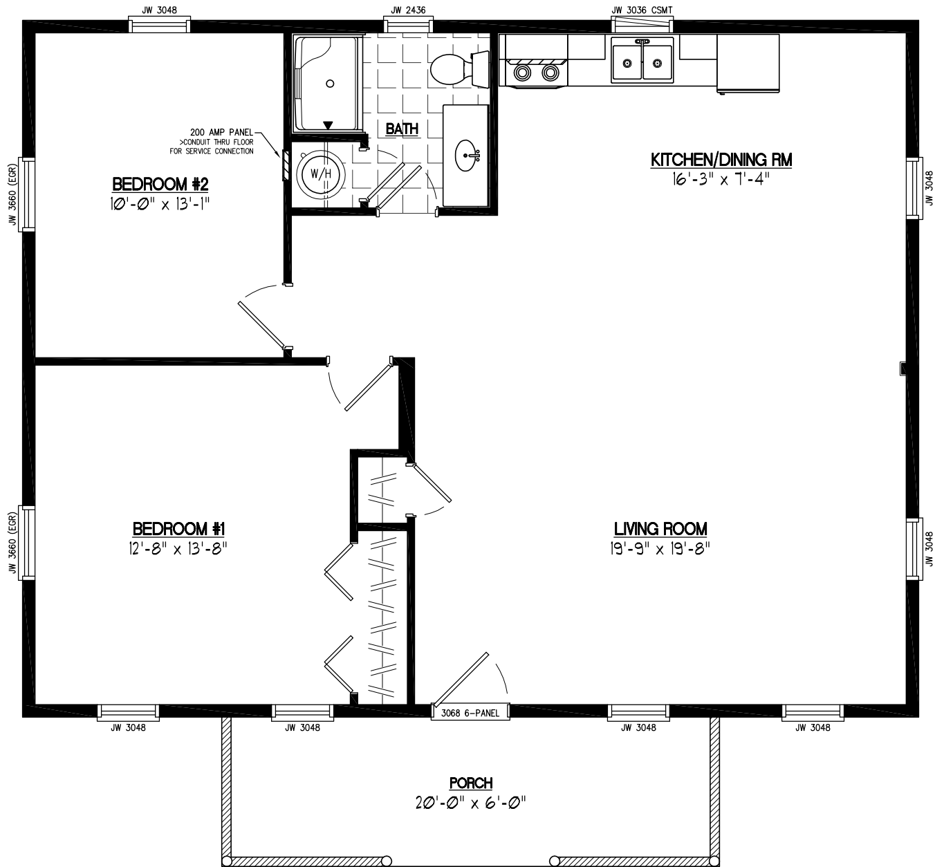
28x36 PIONEER Plan #28PR1202
